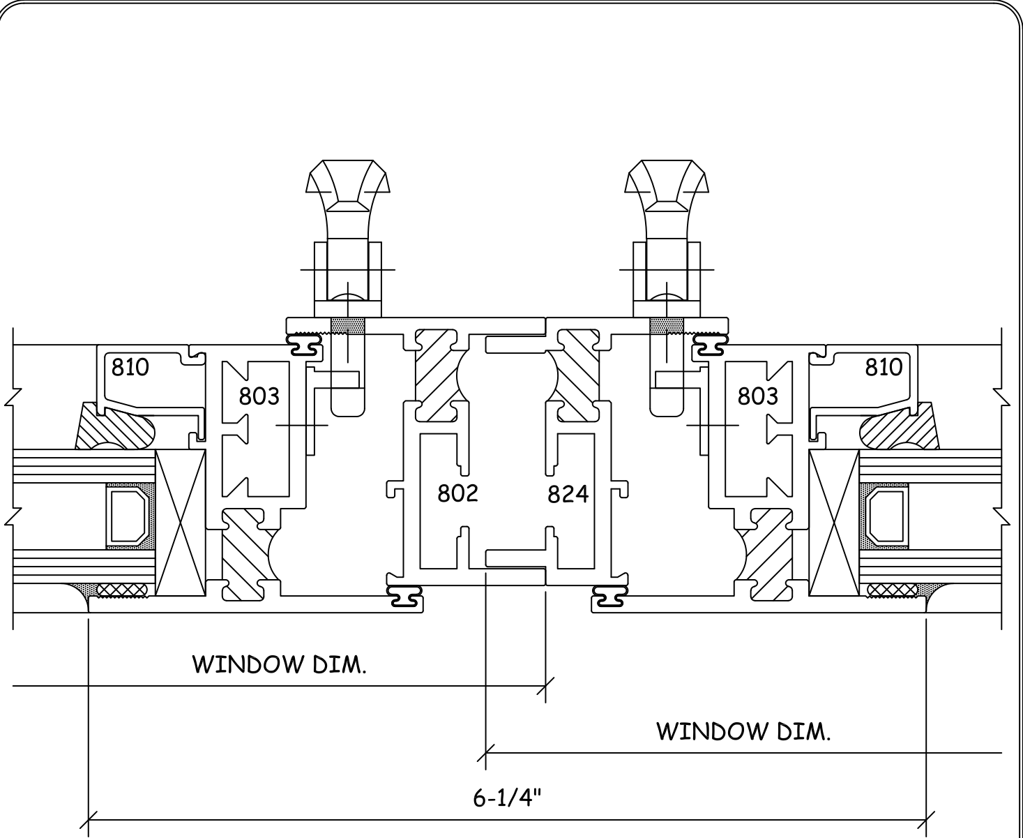
1 8F7 VERTICAL SIDE-STACK CASEMENT/CASEMENT
