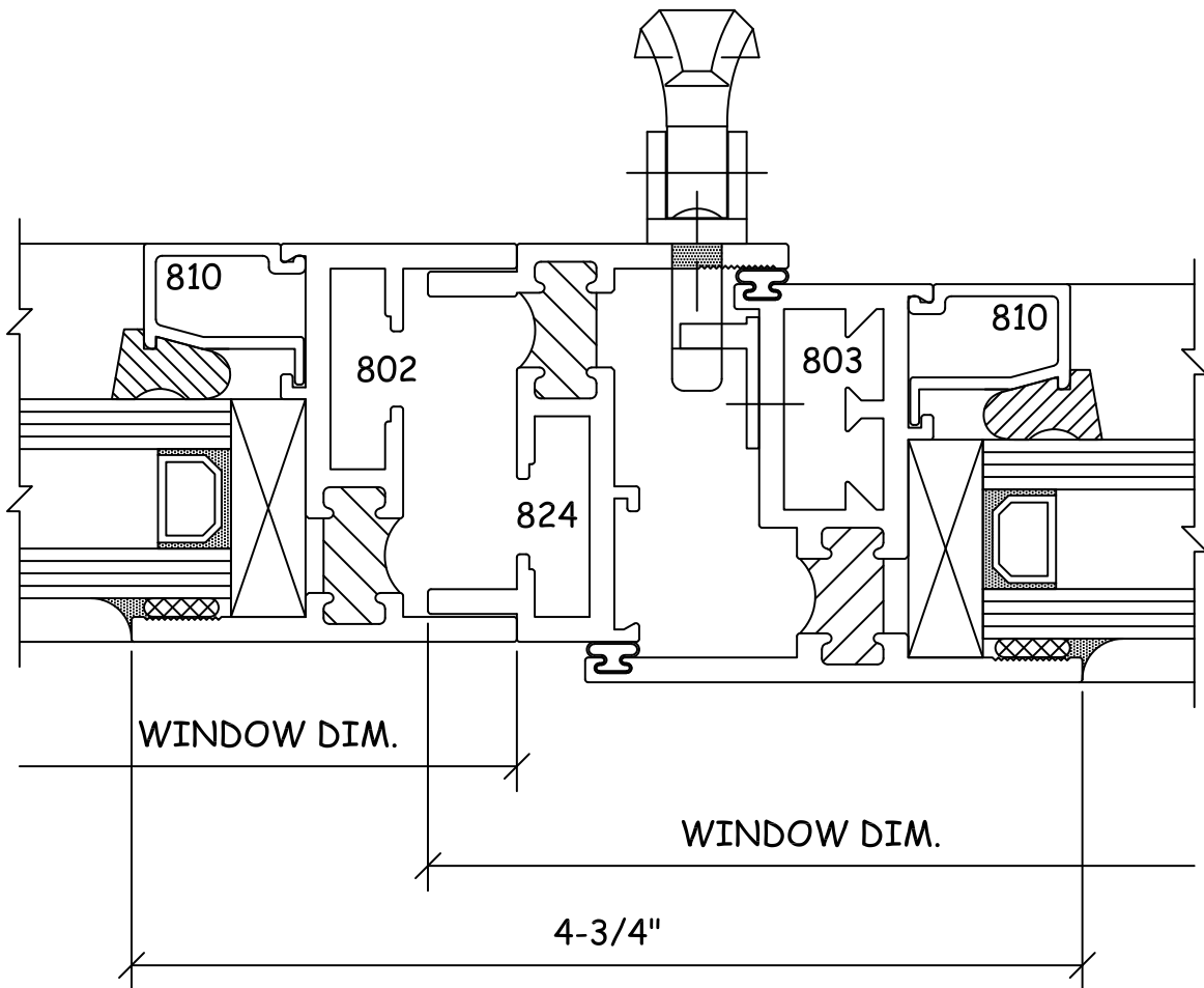
1 VERTICAL SIDE-STACK 8F6 FIXED/CASEMENT
