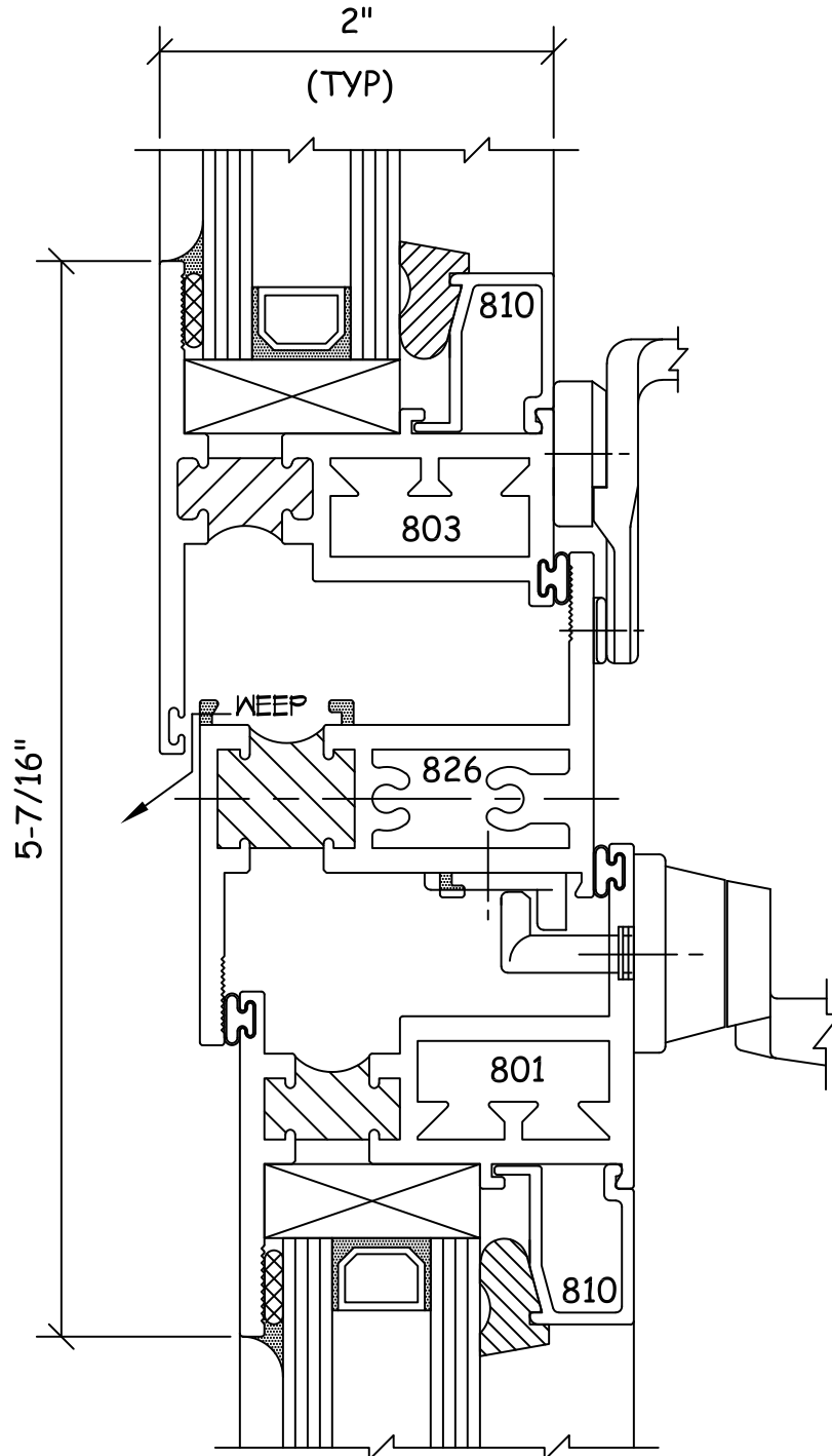
1 HORIZONTAL MUNTIN PROJECT-OUT/PROJECT-IN 8E3
