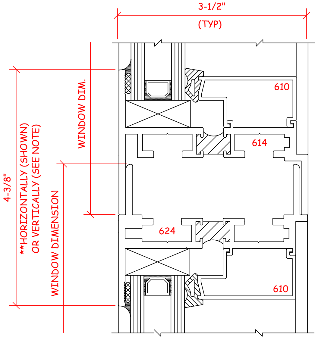
1 HORIZONTAL STACK MULL 6F1 FIXED/FIXED
