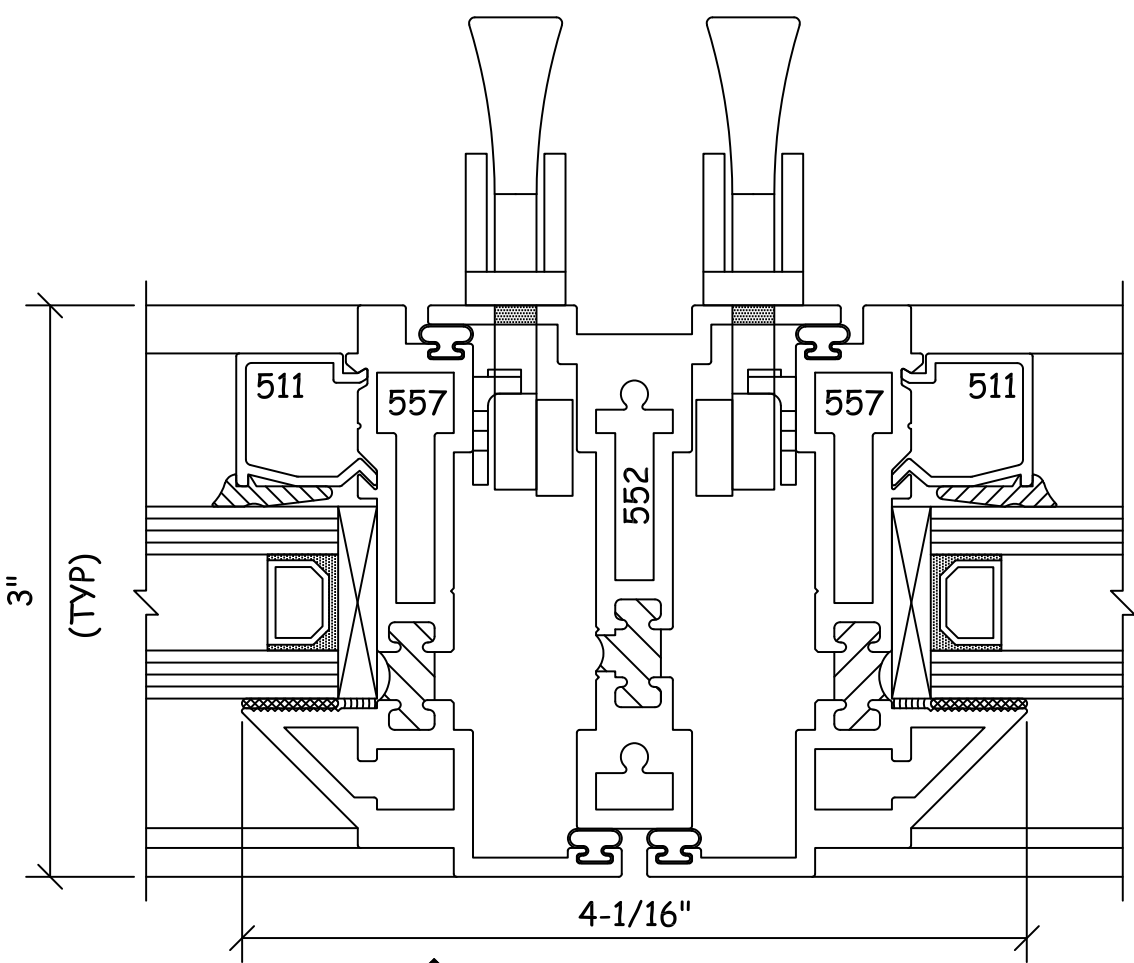
5 VERTICAL MUNTIN 5I3
