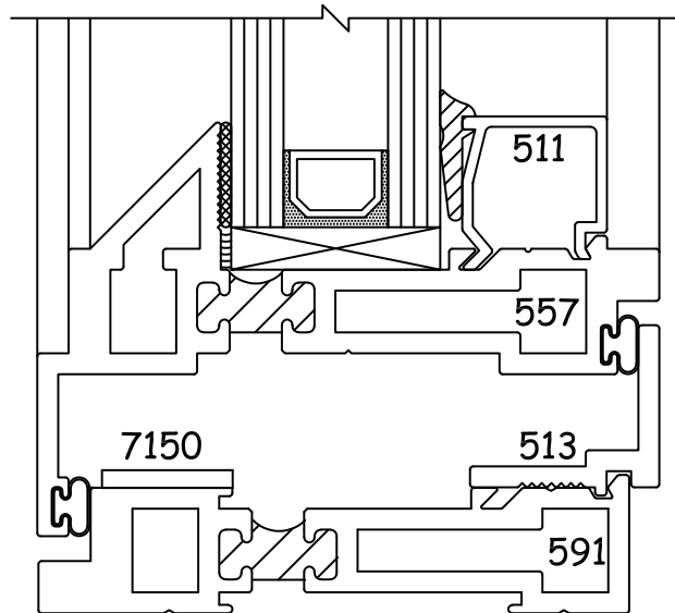
VENT SILL FIXED-CASEMENT 10 5D6
