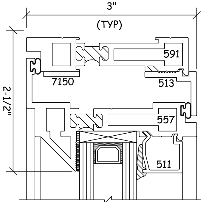
VENT HEAD FIXED-CASEMENT 9 5D6
