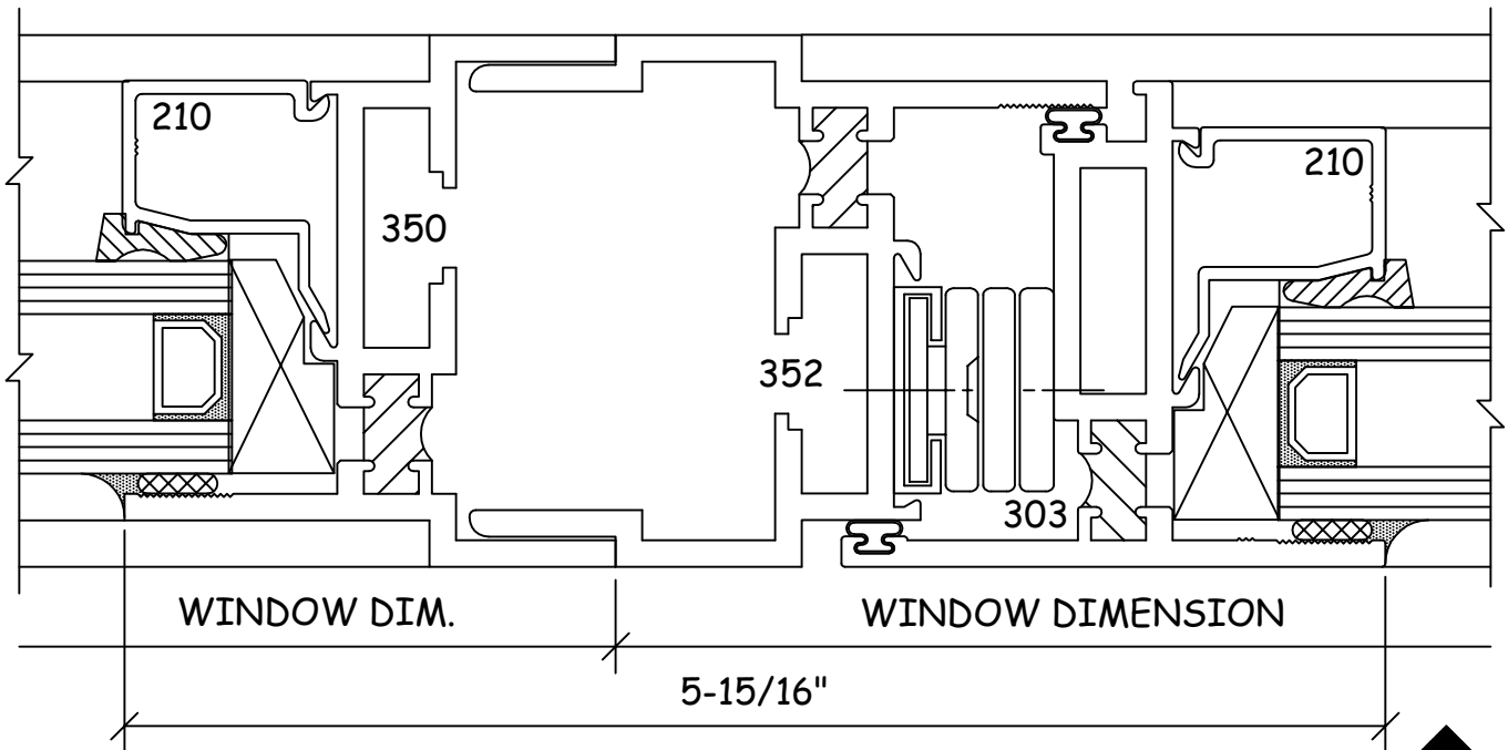
VERTICAL SIDE-STACK FIXED/PROJECT-OUT
