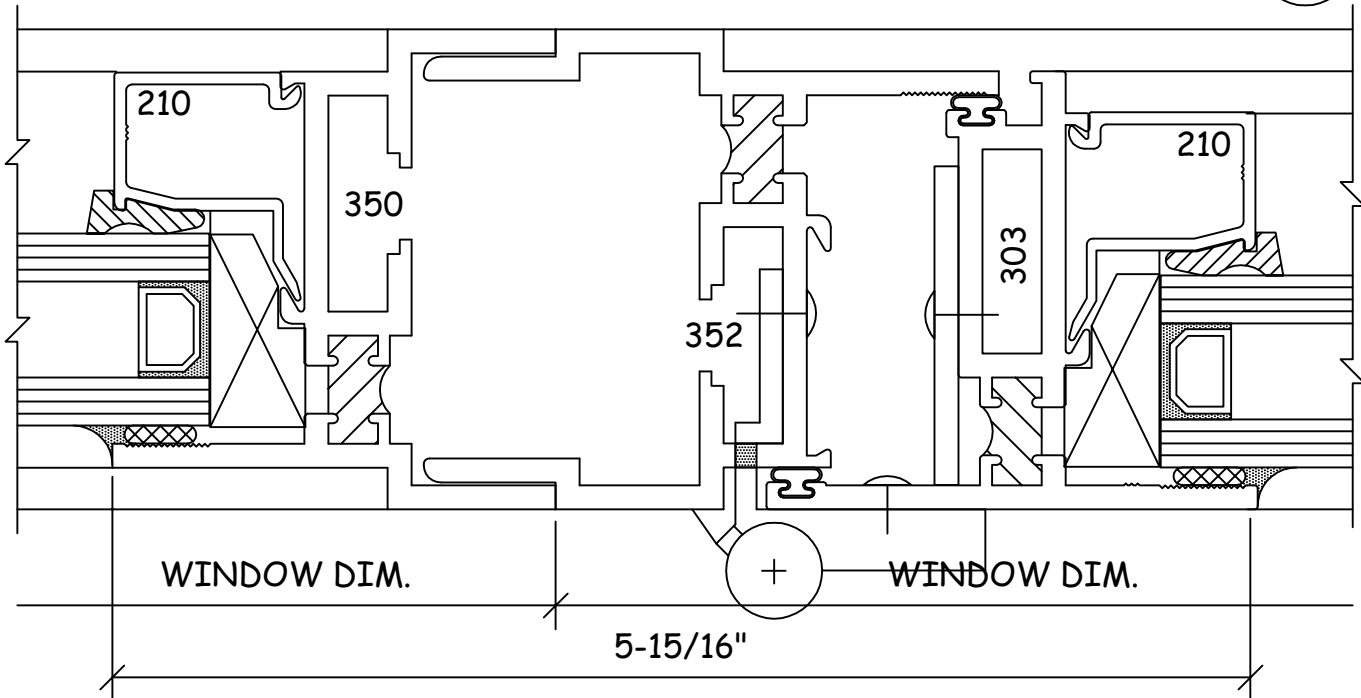
2 VERTICAL SIDE-STACK FIXED/CASEMENT
