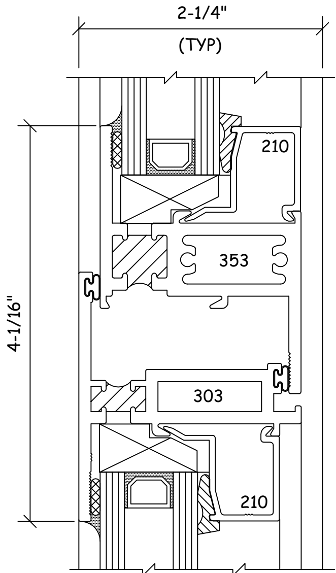
5 35C3 HORIZONTAL MUNTIN PROJECT-OUT/PROJECT-OUT
