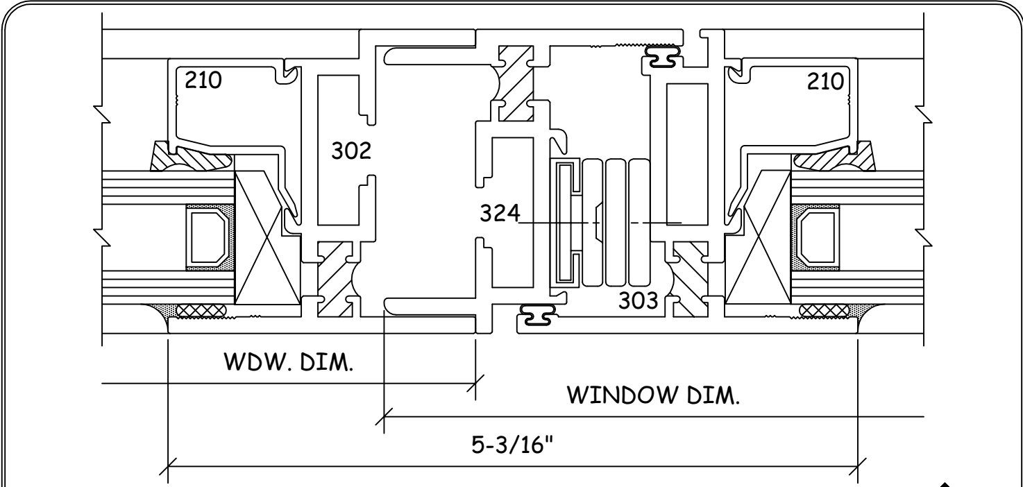
VERTICAL SIDE-STACK MULL FIXED/PROJECT-OUT 1 3F4
