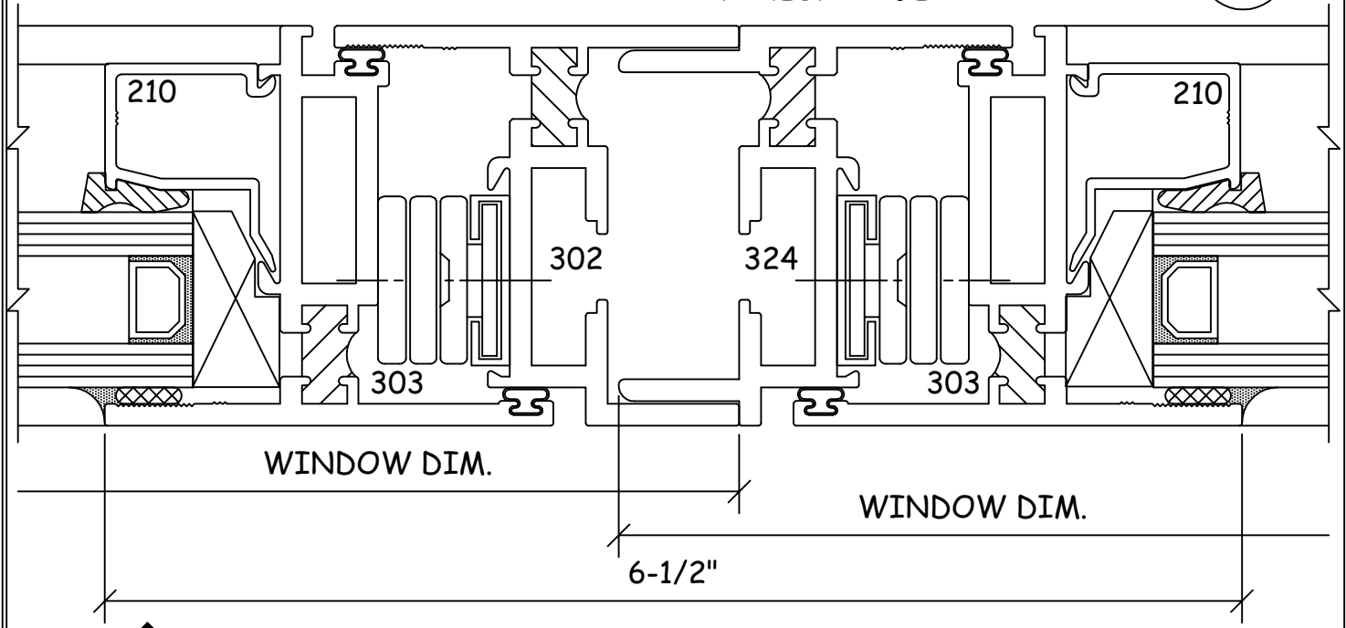
2 3F4 VERTICAL SIDE-STACK MULL PROJECT-OUT/PROJECT-OUT
