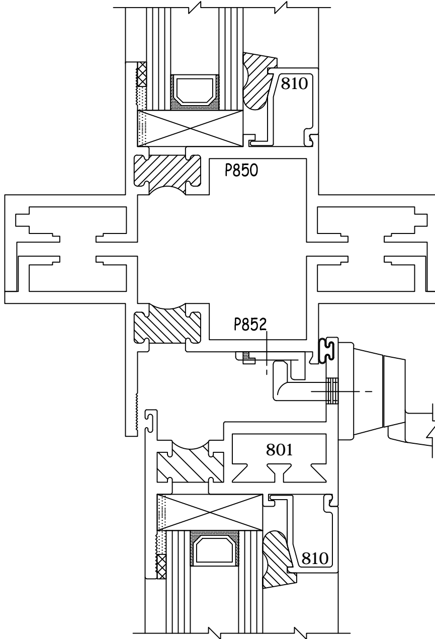
1 HORIZONTAL STACK 85F5 FIXED/PROJECT-IN
