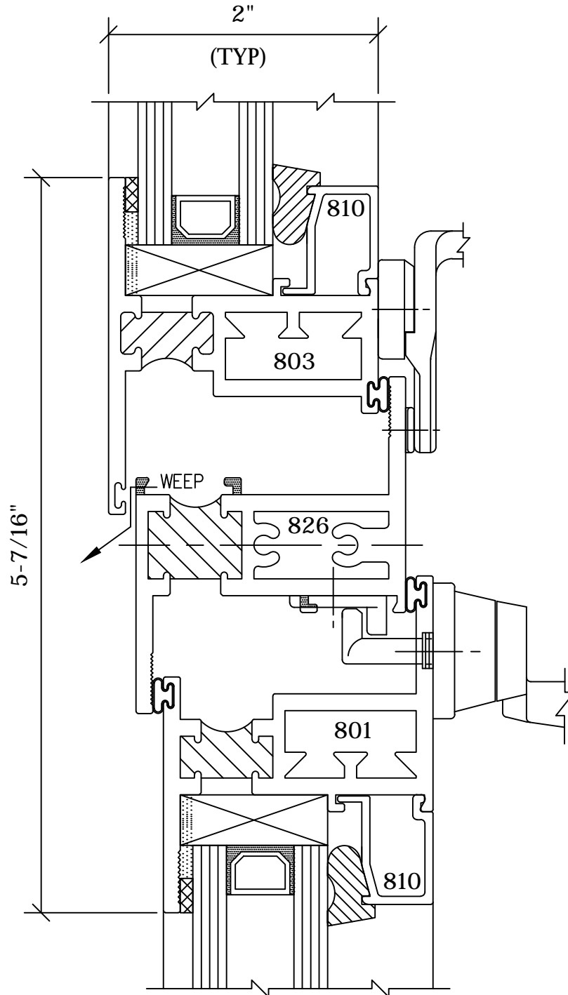
1 HORIZONTAL MUNTIN 8E3 PROJECT-OUT/PROJECT-IN
