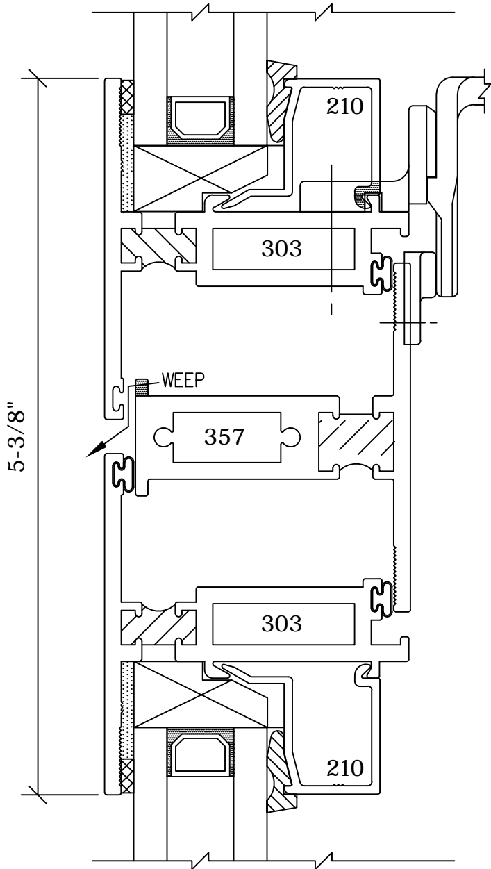
5 35C3 HORIZONTAL MUNTIN PROJECT-OUT/PROJECT-OUT
