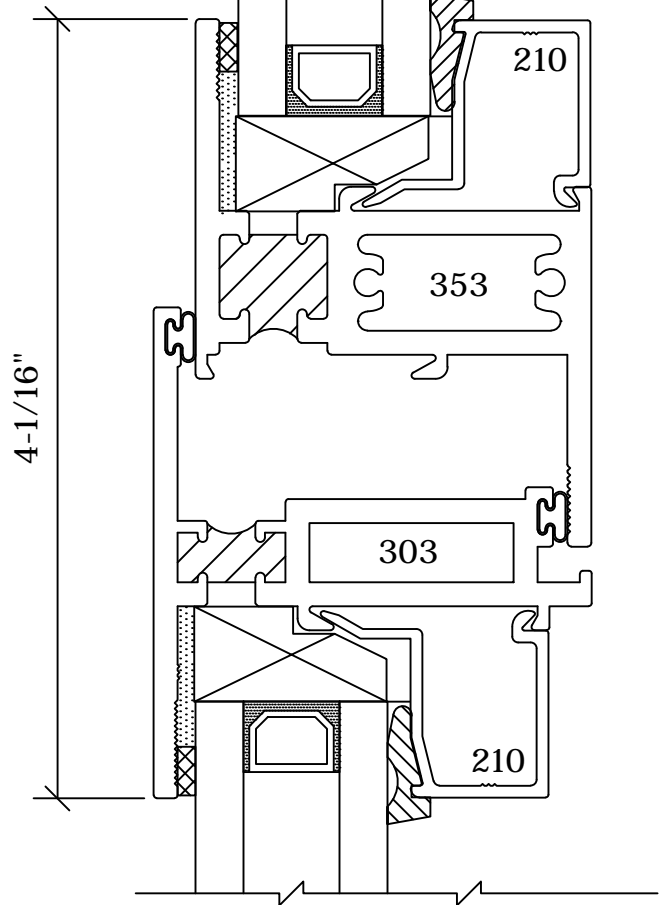
5 35C3 HORIZONTAL MUNTIN PROJECT-OUT/PROJECT-OUT
