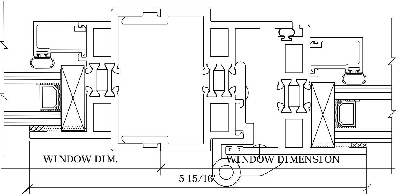
2 VERTICAL SIDE-STACK FIXED/CASEMENT
